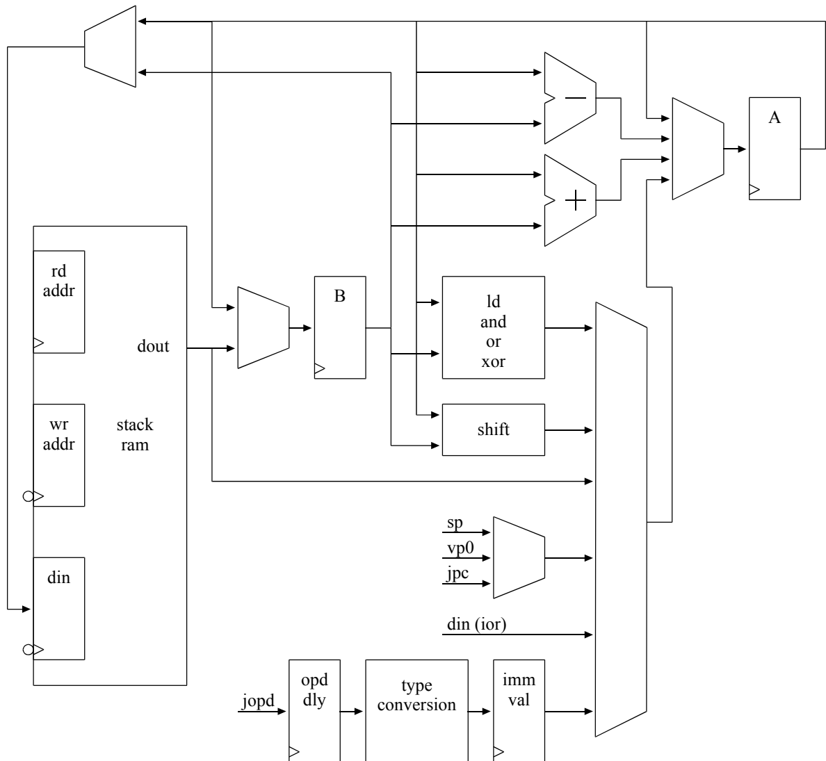
Figure 5: Execute
