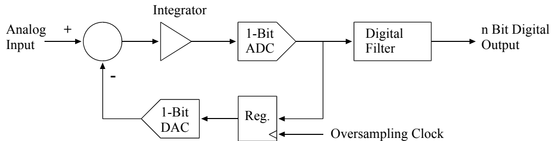
Figure 7: Sigma-Delta ADC
