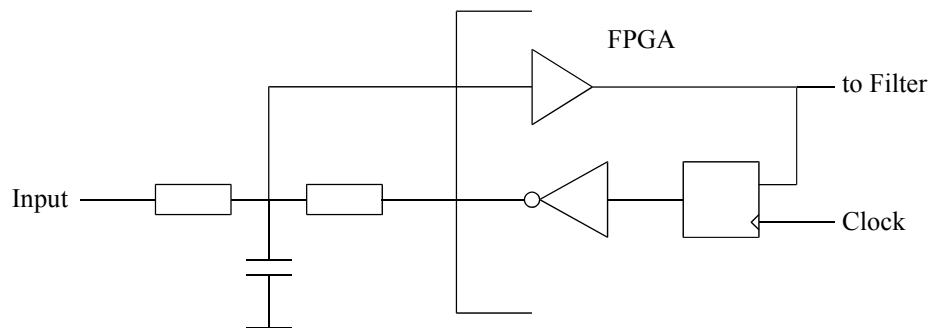
Figure 8: Minimal ADC
