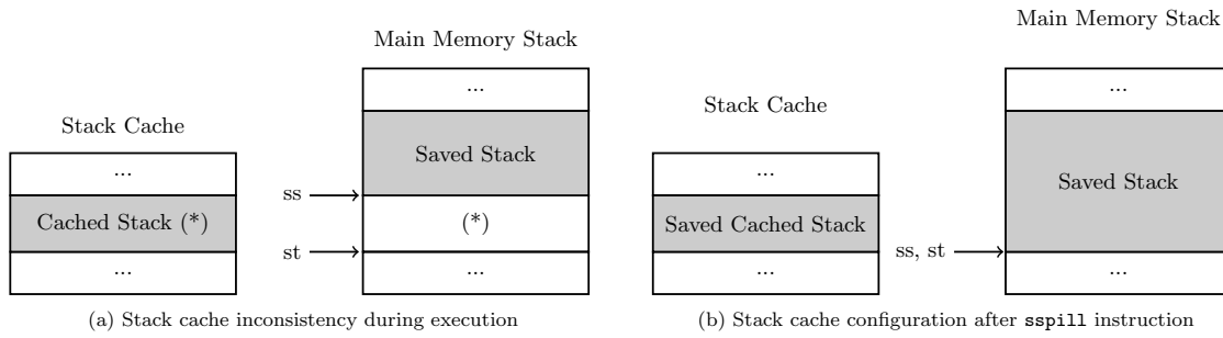
Figure 1: Stack cache manipulation through the sspill instruction
